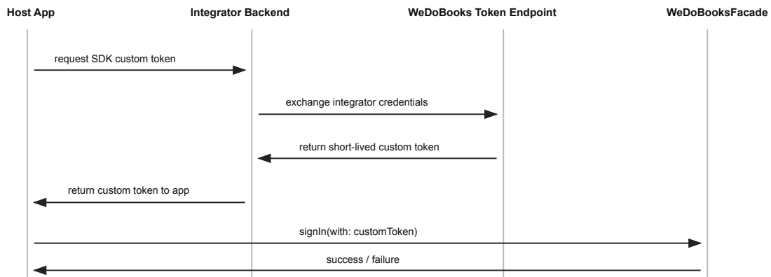
Figure 1: Setup and auth sequence
